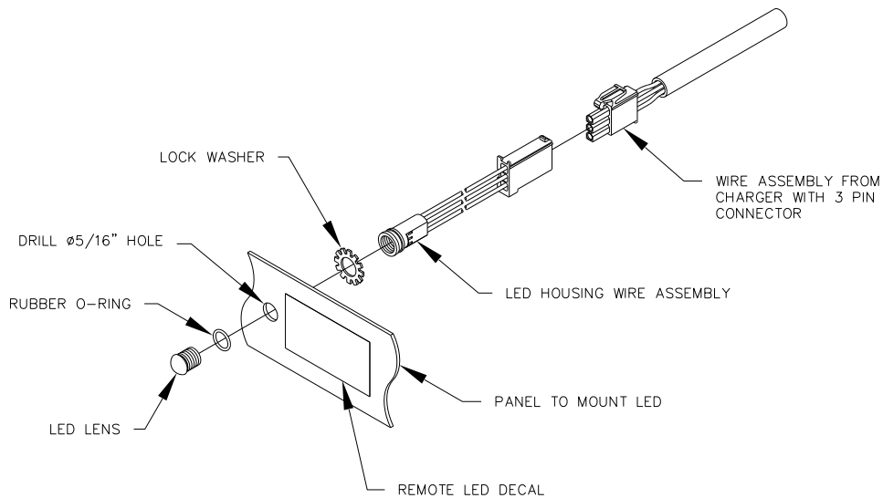
Figure 2-2: Remote LED Installation
