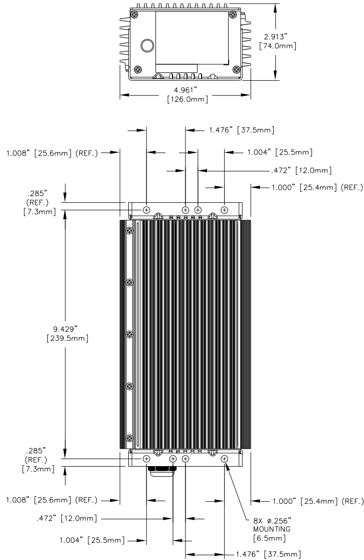
Figure 2-1: Charger Dimensions and Mounting Slot Locations
