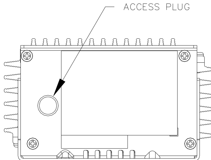
Figure 3-1: Location of the Access Plug for the Active Charge Profile DIP Switch
